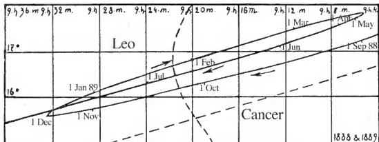
Fig. 3.19. Looping trajectory of Saturn between Cancer and Leo in 1888 and 1889. Taken from [542], page 12, ill. 4.
