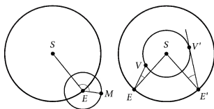
Fig. 2.1. Lunar elongation is the angle between the vectors ES and EM . The elongation of Venus is the angle between ES and EV . The maximal elongation of Venus is the angle between E'S and E'V' .
